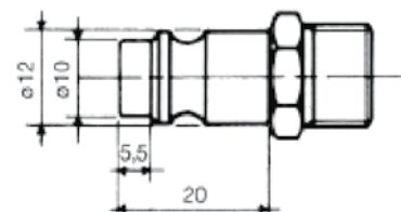
Foro interno d.7,0 mm Internal hole d.7,0 mm
